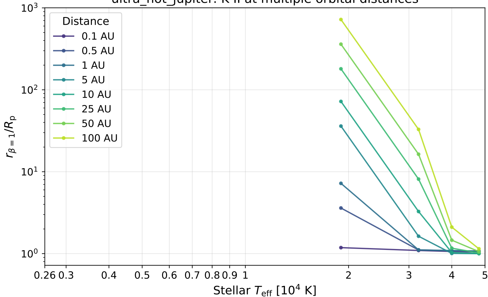
ultra_hot_jupiter: K II at multiple orbital distances
